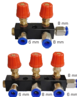
AC-02 / AC-03 AIR CONTROLLER
